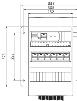
COFFRET DE PROTECTION IT & DELESTAGE PROTECTION & LOAD SHEDDING BOX
