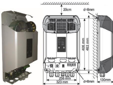
CONVERTISSEUR 24Vdc/230Vac 24Vdc/230Vac INVERTER
