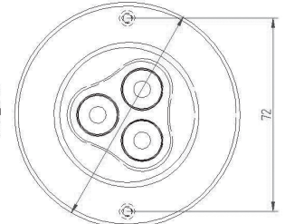
Montage arrière Rear mounting
